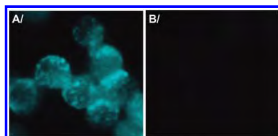
Figure 5. (A) PC-12 cells incubated with 20 \mu M Mini202 for 1 h. (B) PC-12 cells preincubated with VMAT1 inhibitor reserpine (1 \mu M, 1 h) followed by 20 \mu M Mini202 treatment for 1 h. The uptake of Mini202 was blocked by reserpine. \lambda_{ex} = 350 \pm 25 nm, \lambda_{em} = 460 \pm 25 nm.
