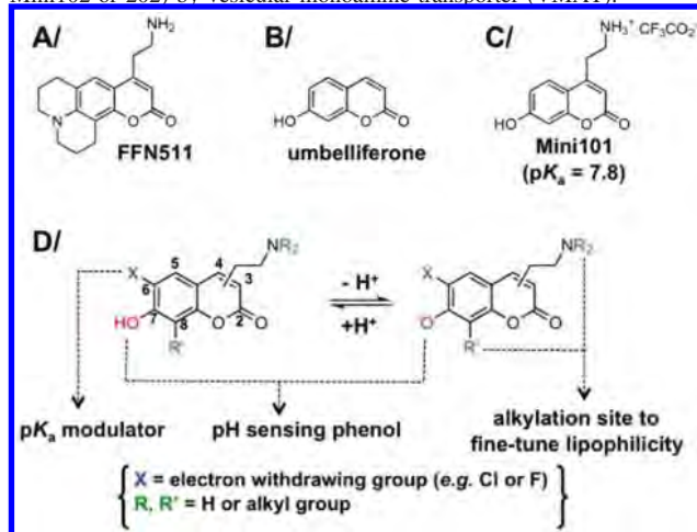
Figure 2. Design of pH-responsive FFNs based on the coumarin nucleus. (A) Structure of FFN511, the first example of FFN probes. (B) Structure of umbelliferone. (C) Chemical structure of Mini101. (D) The key structural elements for optimization of photophysical, physical, and functional properties of pH-responsive FFNs.
